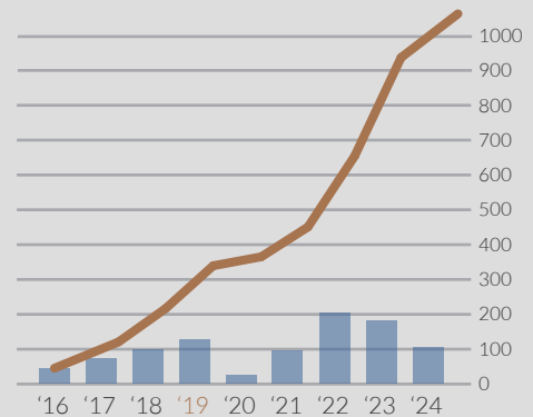
Wells Year-over-Year
